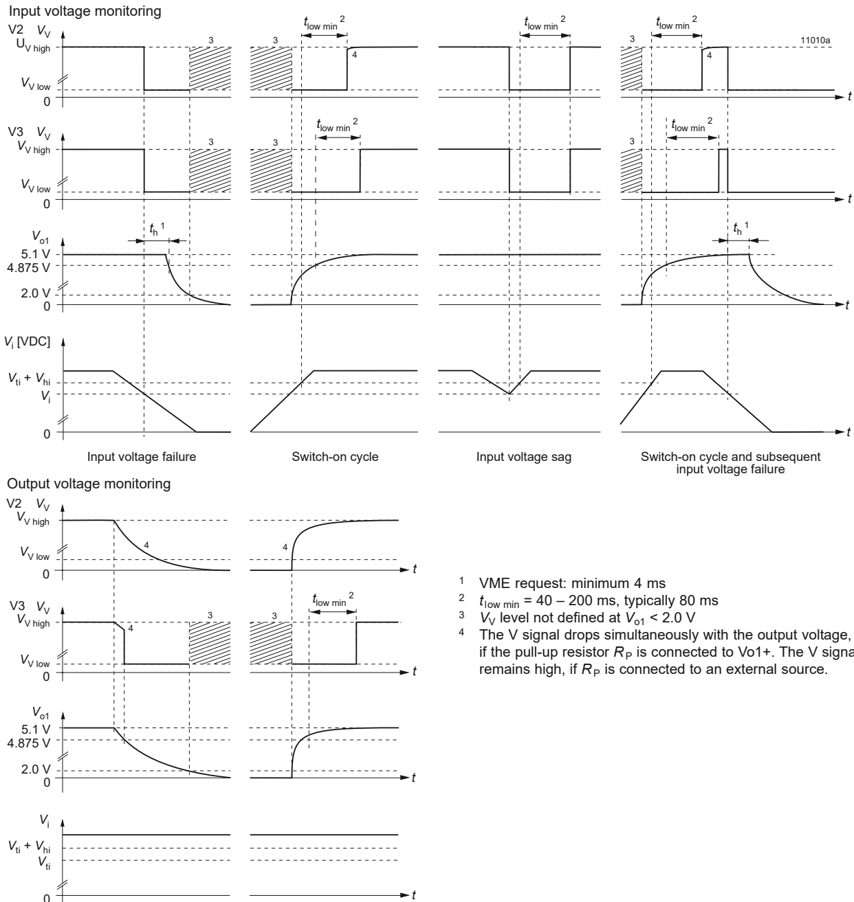
Fig. 26 Relationship between V_i , V_{01} , V_V , I_V , and V_{01}/V_{0\text{ nom}} versus time.
