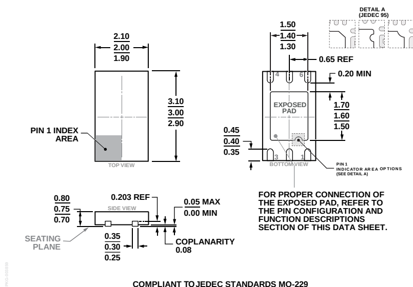
Figure 55. 6-Lead Lead Frame Chip Scale Package [LF CSP] 2.00 × 3.00 mm Body and 0.75 mm Package Height (CP-6-5)
