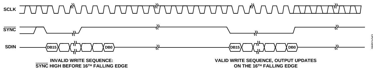
Figure 44. SYNC Interrupt Facility
