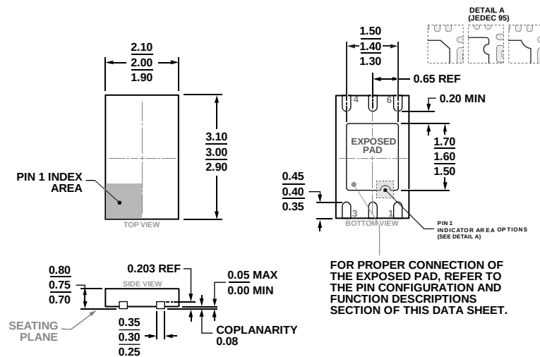
COMPLIANT TO JEDEC STANDARDS MO-229 Figure 55. 6-Lead Lead Frame Chip Scale Package [LFCSP] 2.00 x 3.00 mm Body and 0.75 mm Package Height (CP-6-5) Dimensions shown in millimeters
