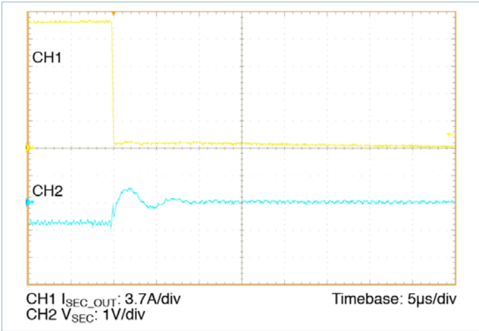
Figure 16 — 16.9 – 0A transient response: C_{PRI\_IN\_EXT} = 2.2\mu F , no external C_{SEC\_OUT\_EXT}
