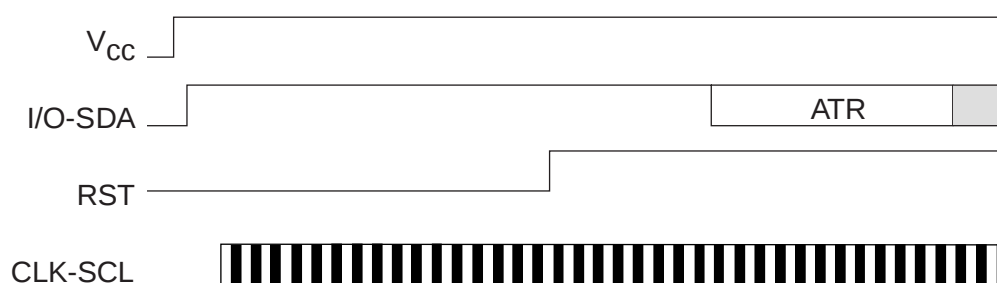
Figure 11-2. Asynchronous T = 0 Protocol (Gemplus Patent)
