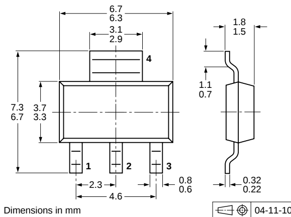
Fig 13. Package outline SOT223 (SC-73)
