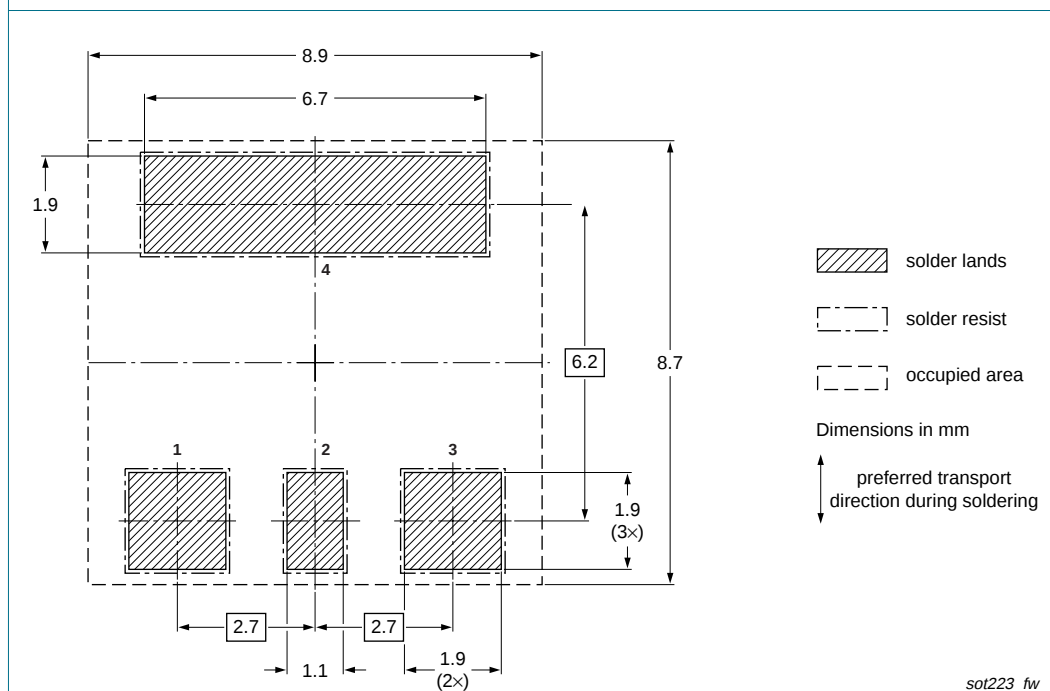
Fig 15. Wave soldering footprint SOT223 (SC-73)
