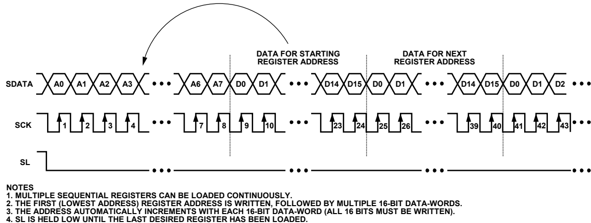
Figure 17. Continuous Serial Write Operation
