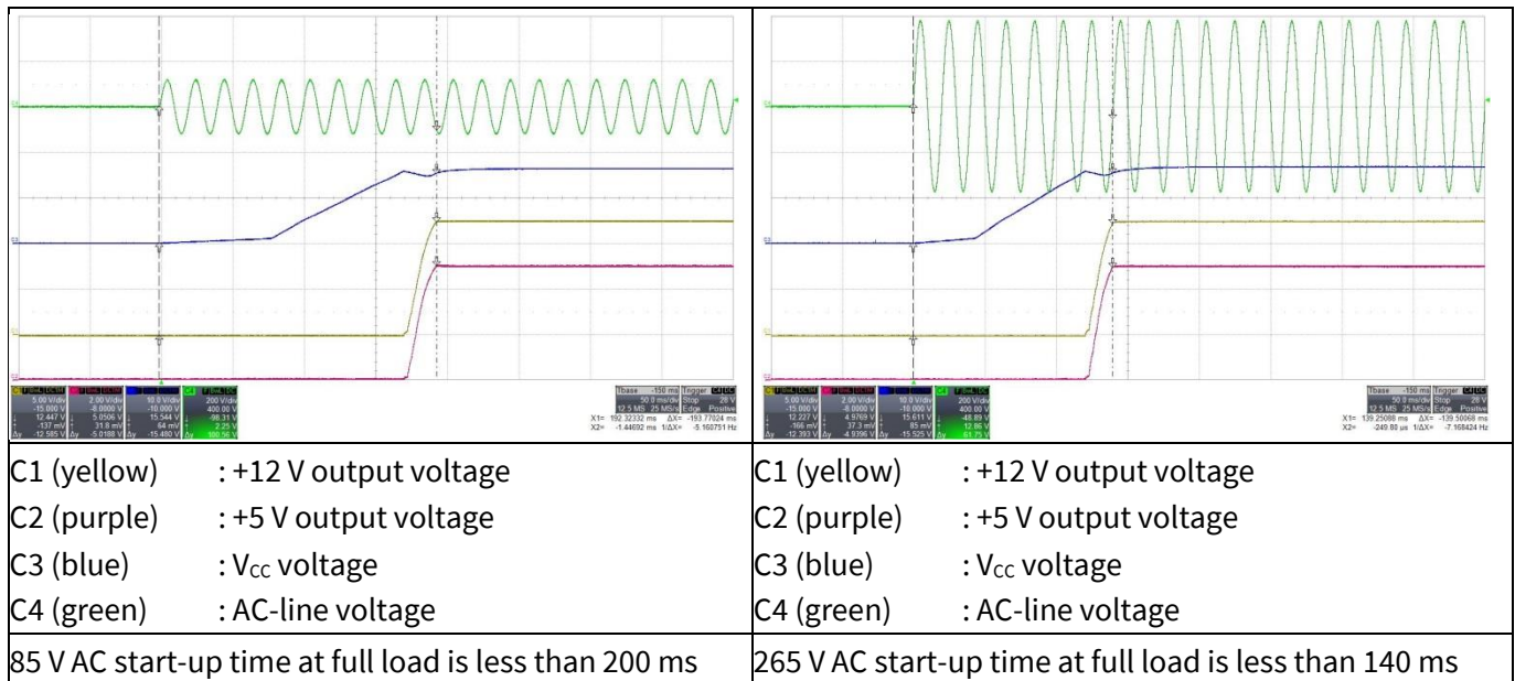
Figure 21 Start-up
