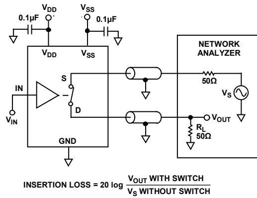
Figure 24. Bandwidth
