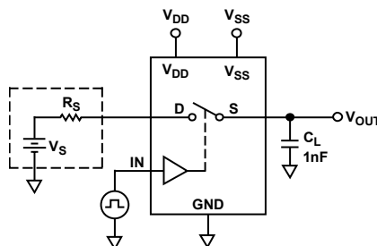
Figure 21. Charge Injection
