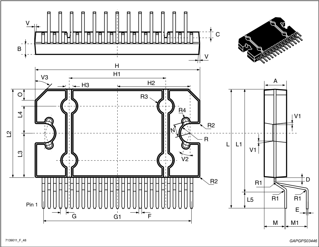
Figure 27. Flexiwatt 27 (vertical) package outline
