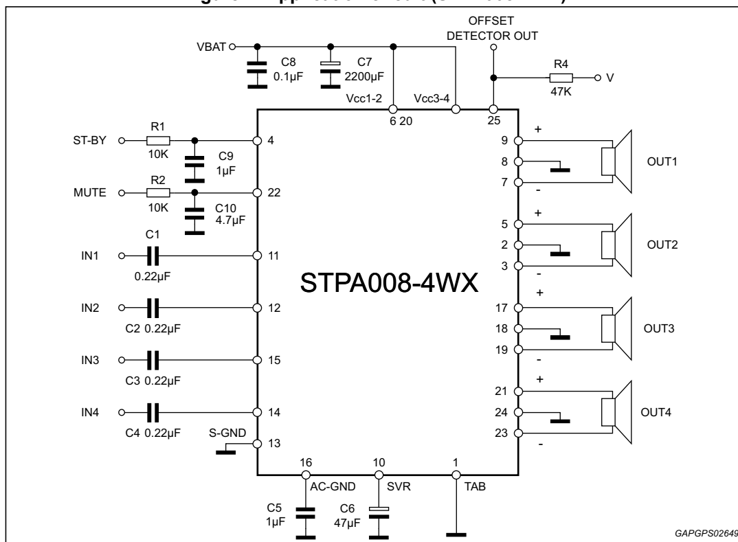
Figure 2. Application circuit (STPA008-4WX)
