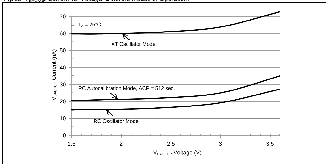
Typical V_{\text{BACKUP}} Current vs. Voltage, Different Modes of Operation:
