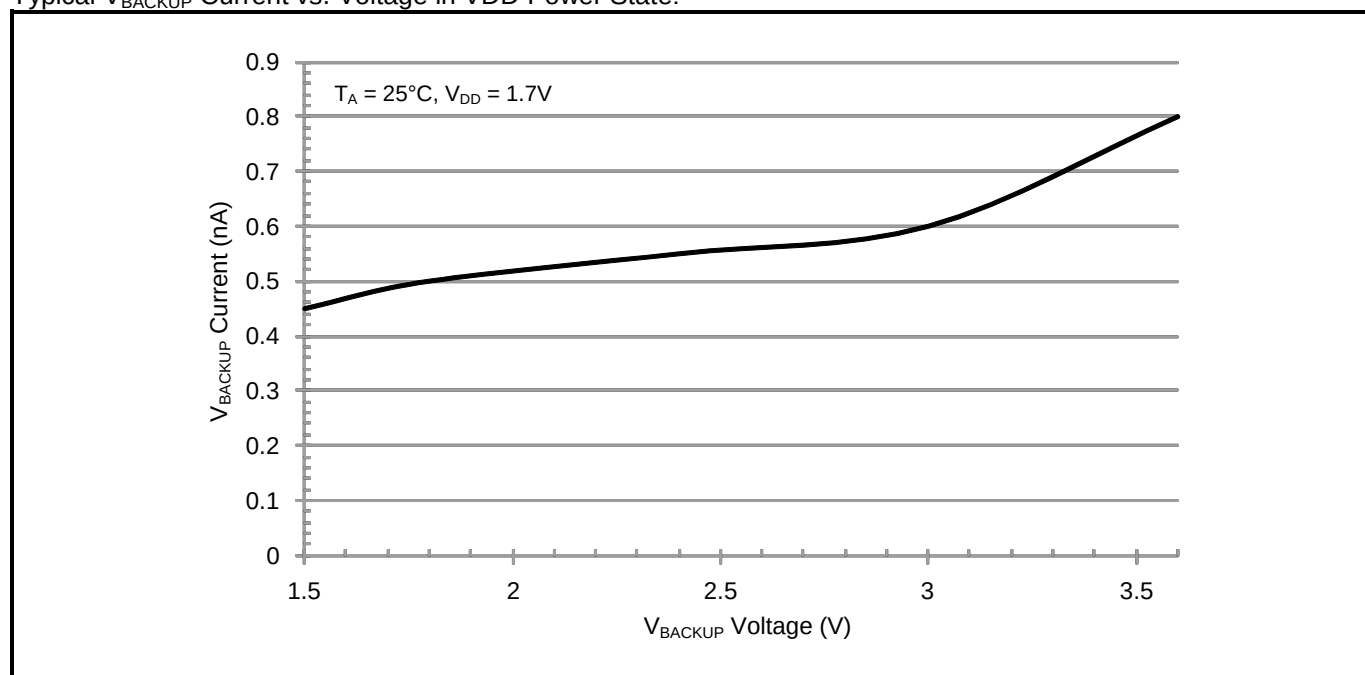
Typical V_{\text{BACKUP}} Current vs. Voltage in V_{\text{DD}} Power State:
