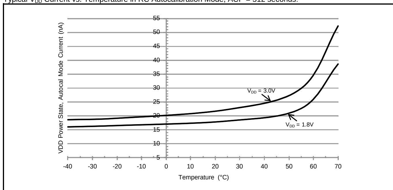
Typical V DD Current vs. Temperature in RC Autocalibration Mode, ACP = 512 seconds:
