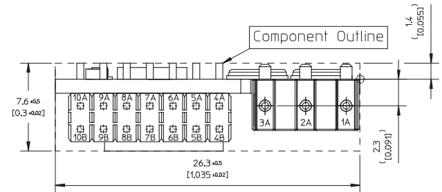
BOTTOM VIEW Pin positions according to recommended footprint
