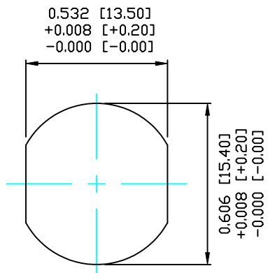
PANEL CUTOUT
