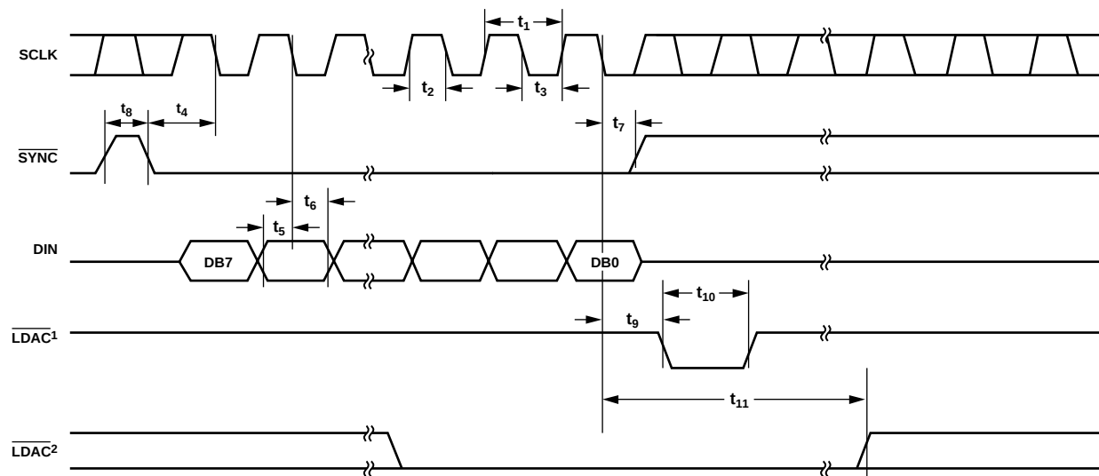
Figure 2. Timing Diagram
