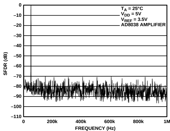
Figure 24. Wideband SFDR, Clock = 2 MHz, f_{OUT} = 50\text{ kHz}
