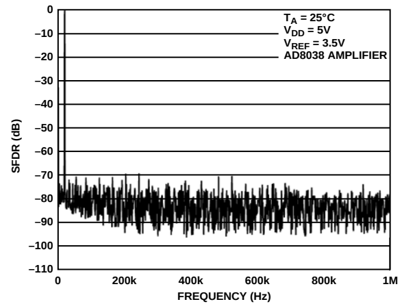
Figure 25. Wideband SFDR, Clock = 2 MHz, f_{OUT} = 20\text{ kHz}
