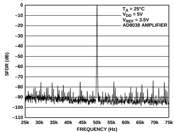
Figure 27. Narrow-Band SFDR, Clock = 2 MHz, f_{OUT} = 50\text{ kHz}
