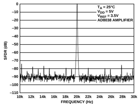
Figure 26. Narrow-Band SFDR, Clock = 2 MHz, f_{OUT} = 20\text{ kHz}
