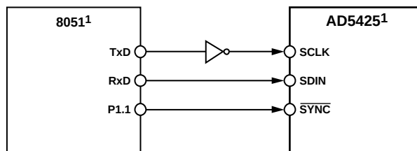
Figure 41. 80C51/80L51 to AD5425 Interface
