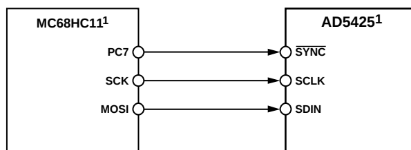
Figure 42. 68HC11/68L11 to AD5425 Interface
