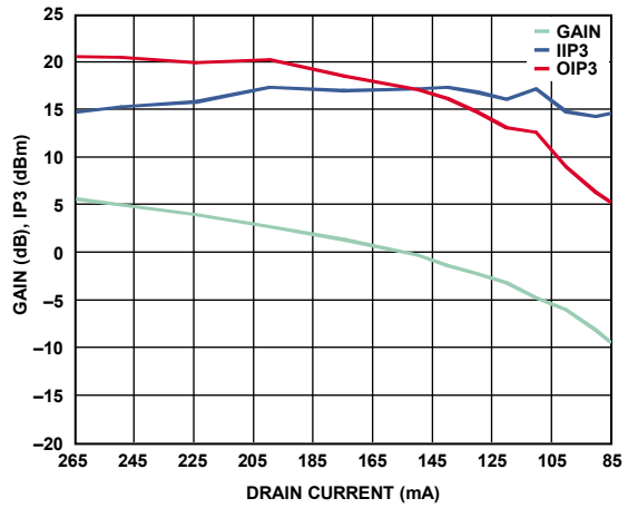
Figure 28. Gain and Input/Output IP3 vs. Drain Current, P_{IN} = -5 dBm/Tone, V_{CTL1}/V_{CTL2} = -1 V, RF = 86 GHz, Drain Current = ( I_{DD1}/I_{DD2} Fixed at 50 mA) + ( I_{DD3} to I_{DD6} Swept)
