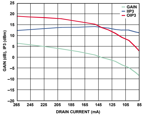
Figure 26. Gain and Input/Output IP3 vs. Drain Current, P_{IN} = -5 dBm/Tone, V_{CTL1}/V_{CTL2} = -1 V, RF = 81 GHz, Drain Current = ( I_{DD1}/I_{DD2} Fixed at 50 mA) + ( I_{DD3} to I_{DD6} Swept)
