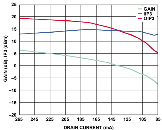
Figure 27. Gain and Input/Output IP3 vs. Drain Current, P_{IN} = -5 dBm/Tone, V_{CTL1}/V_{CTL2} = -1 V, RF = 83.5 GHz, Drain Current = ( I_{DD1}/I_{DD2} Fixed at 50 mA) + ( I_{DD3} to I_{DD6} Swept)
