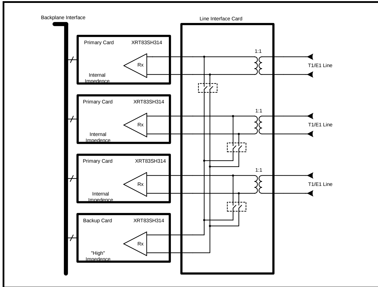
FIGURE 30. SIMPLIFIED BLOCK DIAGRAM OF THE RECEIVE INTERFACE FOR N+1 REDUNDANCY
