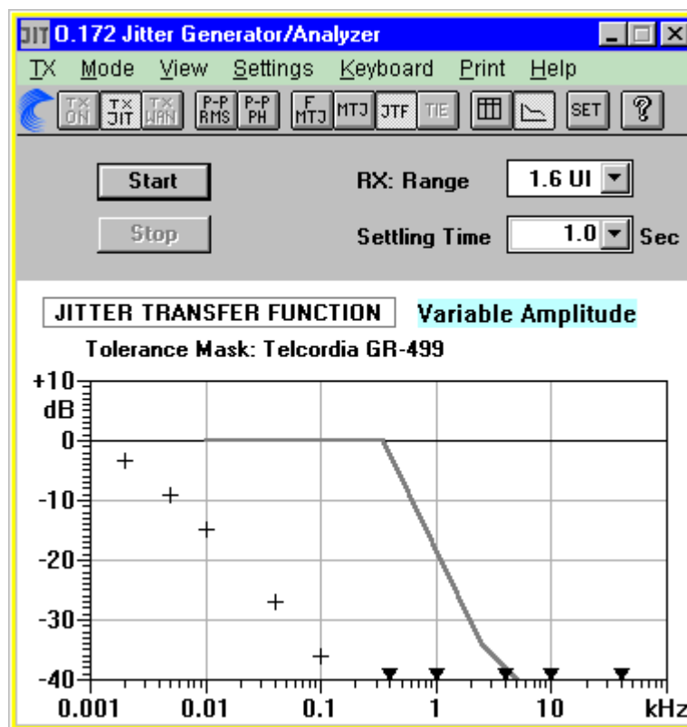
FIGURE 38. JITTER TRANSFER FUNCTION VARIABLE AMPLITUDE - T1 TX 3Hz 32BITS
