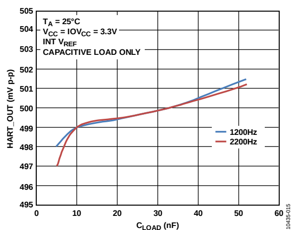
Figure 18. HART_OUT Voltage vs. C_{LOAD}
