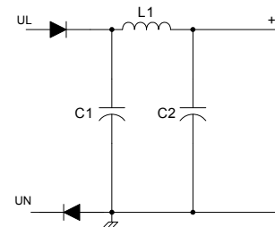
Figure 10: Half-Wave Rectifier
