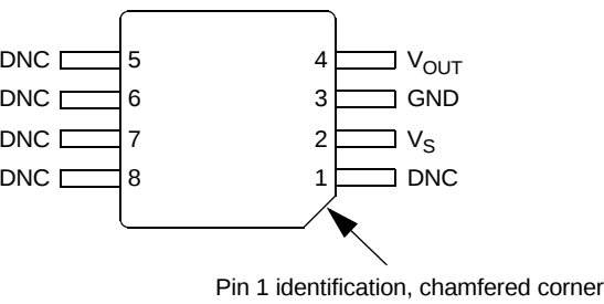
Figure 2. Device pinout (top view)
