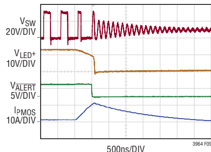
Figure 9. PWMGTG Response to Short Circuit Fault
