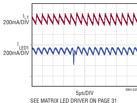
Transient Response at V_{IN} = 34V Zero LED On to One LED On
