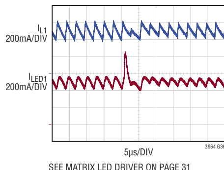
Transient Response at V_{IN} = 34V One LED On to Zero LED On
