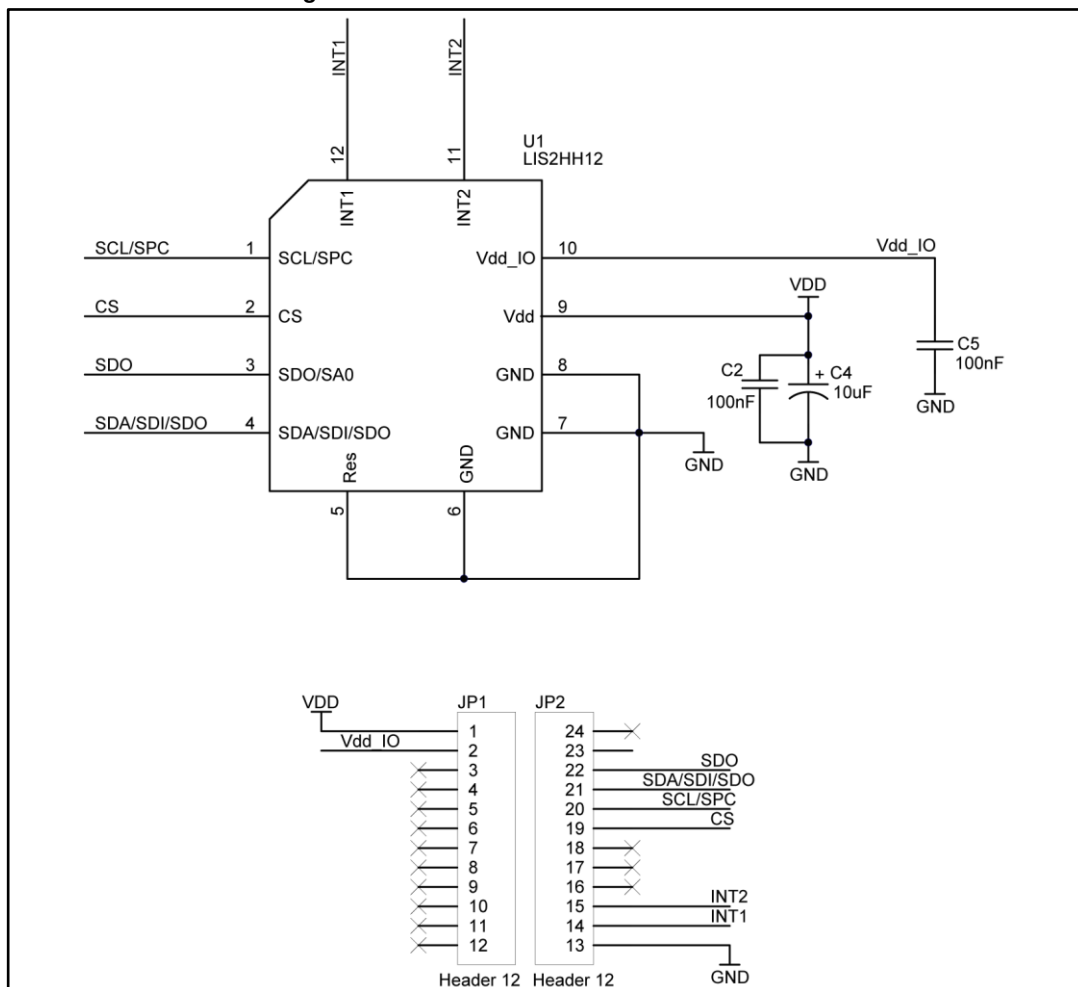
Figure 1: STEVAL-MKI164V1 circuit schematic
