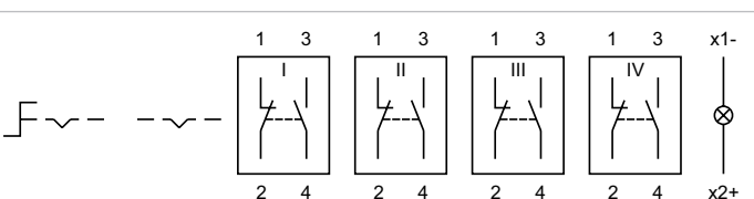
Wiring diagram 28
