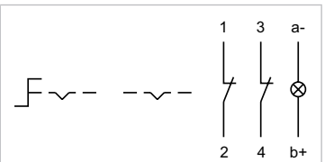
Wiring diagram 18
