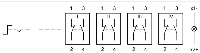
Wiring diagram 14
