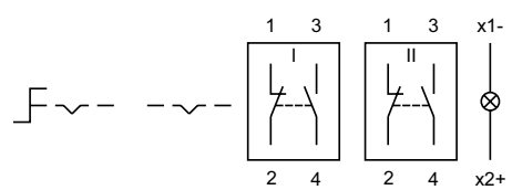
Wiring diagram 26
