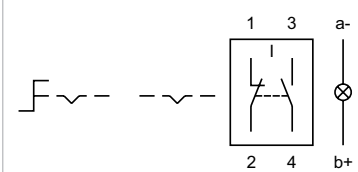
Wiring diagram 23
