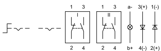
Wiring diagram 25
