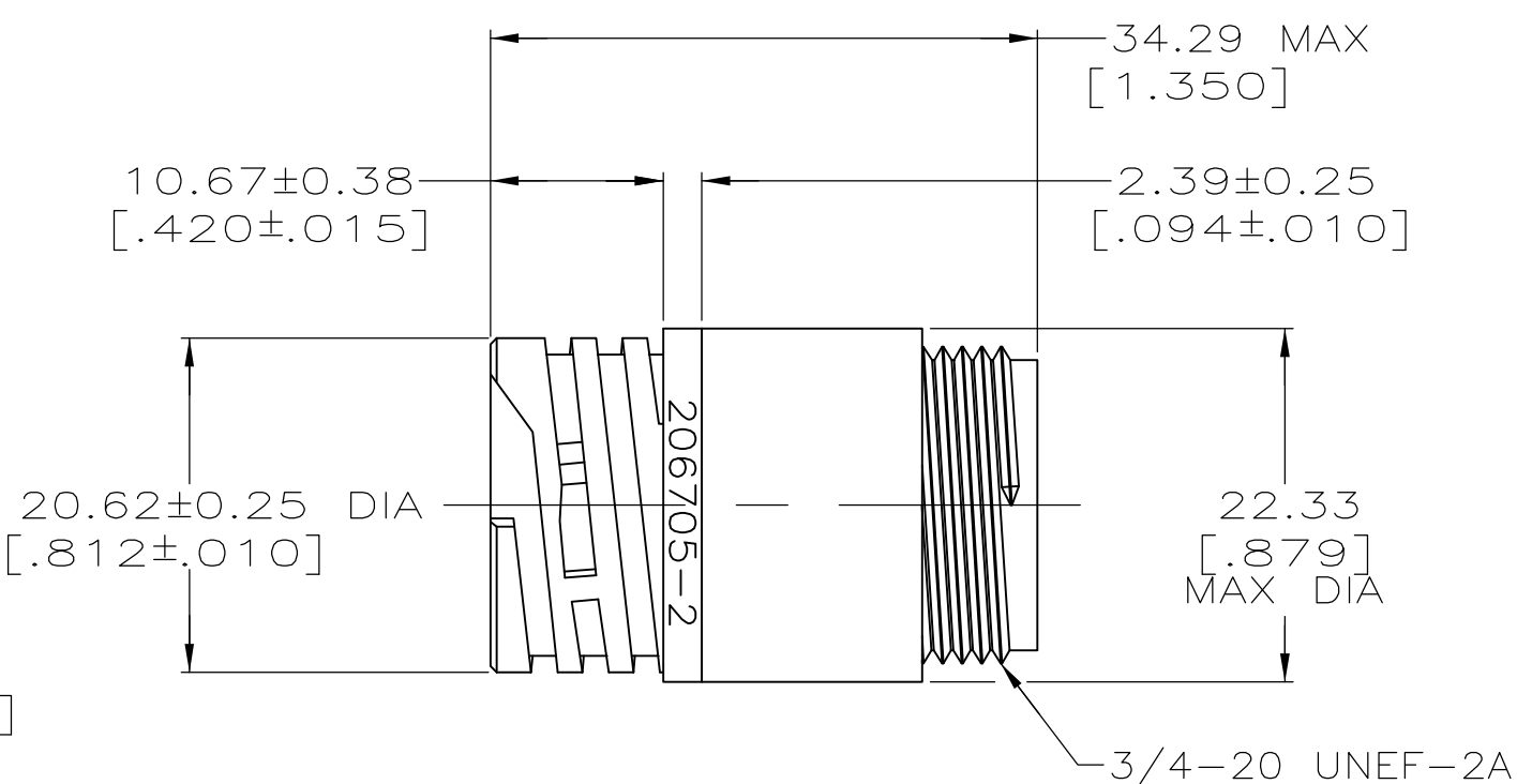
DETAIL A
