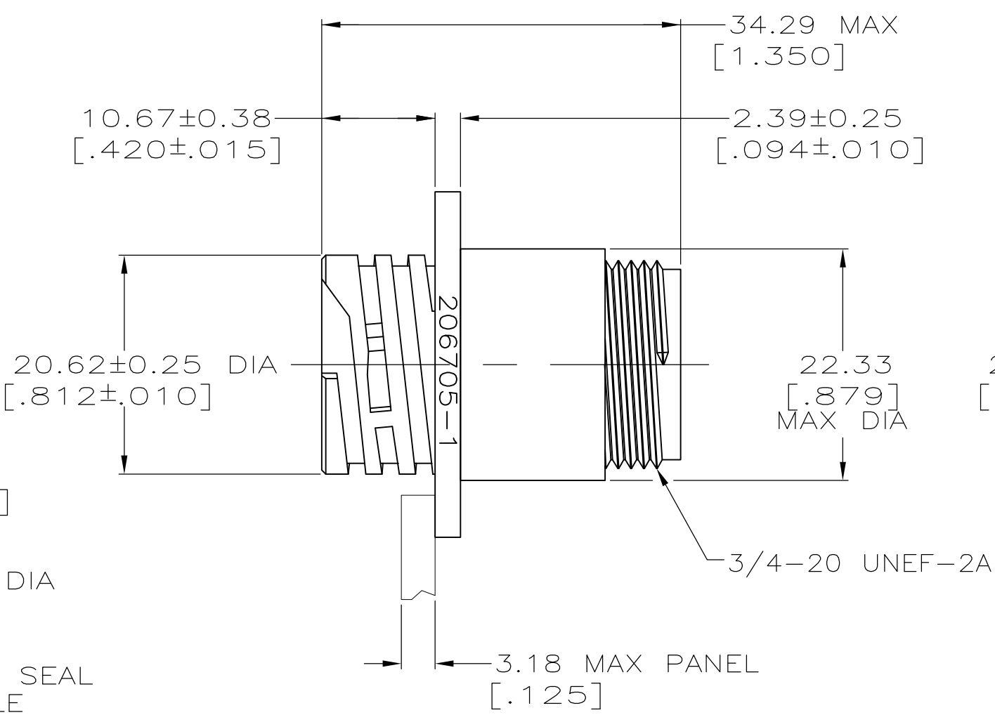
DETAIL A
