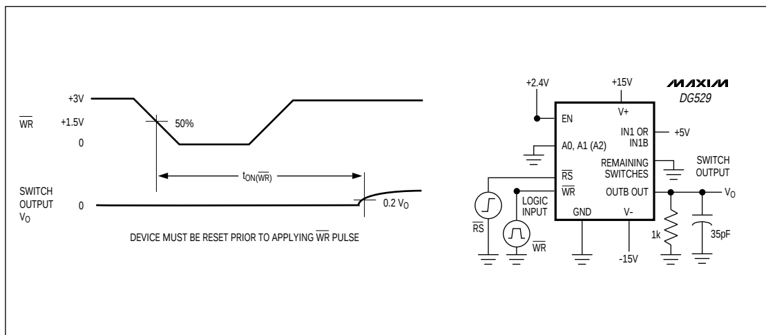
Figure 4. Write Turn-On Time t ON (WR) Test Circuit
