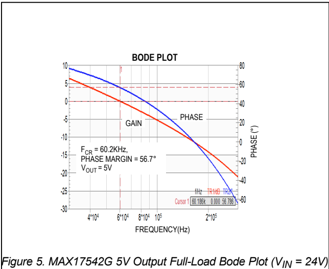
Figure 5. MAX17542G 5V Output Full-Load Bode Plot ( V_{IN} = 24V )
