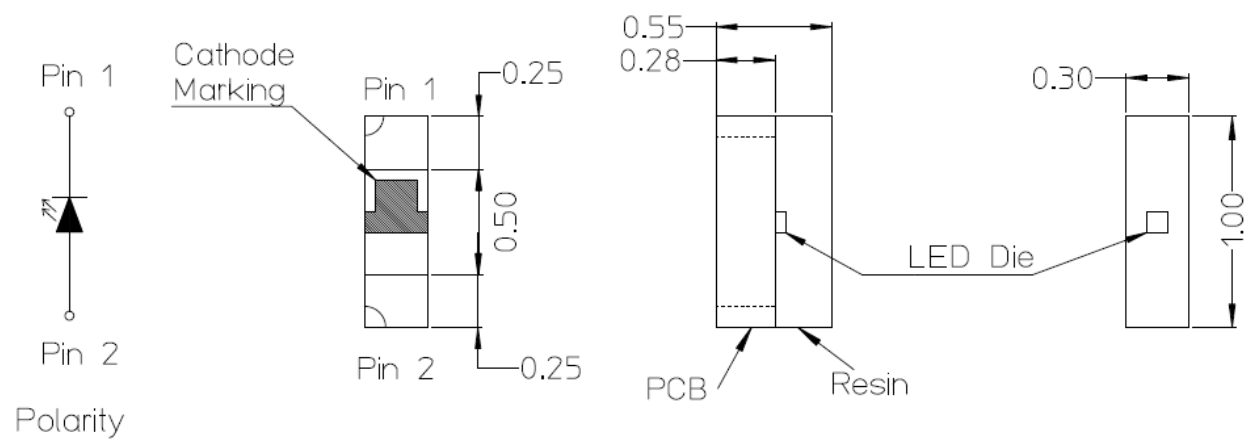
Figure 1: Package Dimensions
