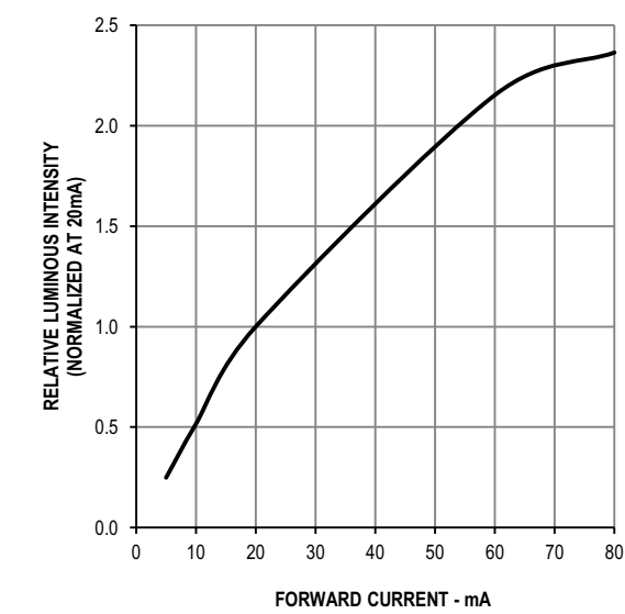
Figure 4: Intensity vs. Forward Current
