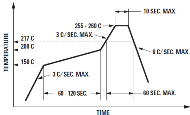
Figure 14: Recommended Reflow Soldering Conditions
