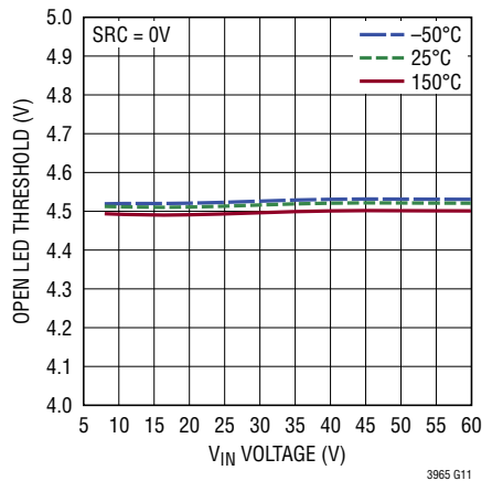
Open LED Threshold Rising vs V_{IN} , Temperature for V_{OTH}[1:0] = 00
