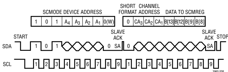
Figure 8. LT3965/LT3965-1 I²C Serial Port SCMODE Write Short Format Protocol
