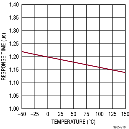
Switch Open LED Protection Response Time vs Temperature
