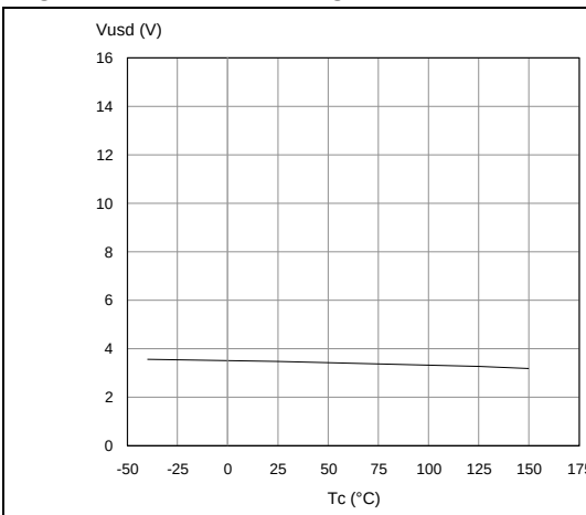
Figure 25. Undervoltage shutdown
