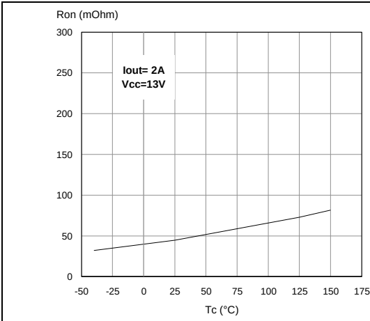
Figure 23. On-state resistance vs T_{case}
