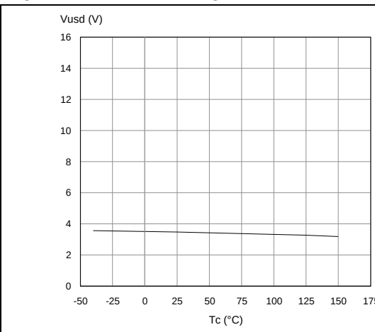
Figure 25. Undervoltage shutdown
