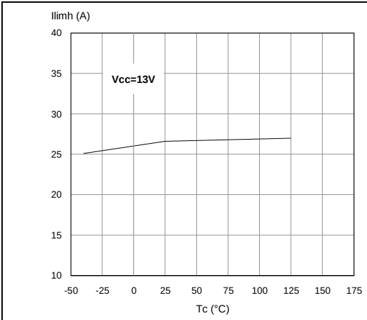
Figure 27. I_{LIMH} vs T_{case}
