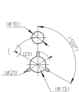
DETAIL "F"
