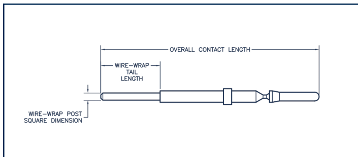
Wire-Wrap Contact
