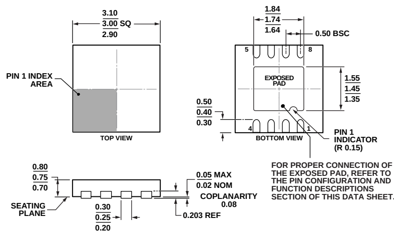
Figure 73. 8-Lead Lead Frame Chip Scale Package [LFCS_P_WD] 3 mm × 3 mm Body, Very Thin, Dual Lead (CP-8-13)
