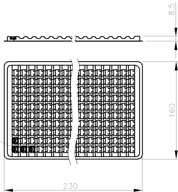
TRAY LAYOUT
