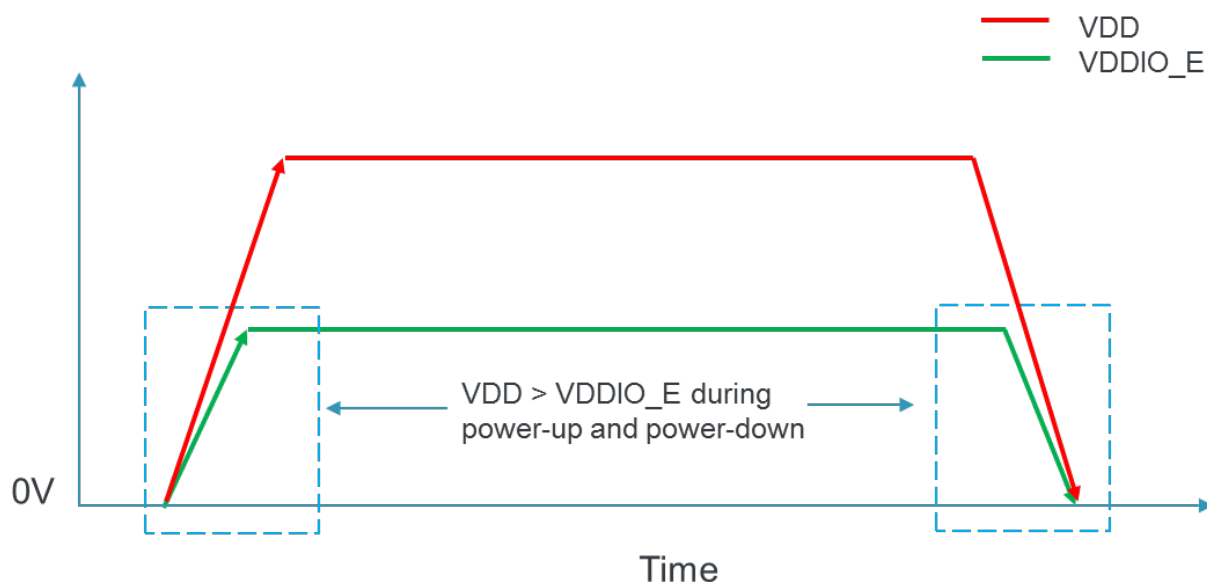
Figure 3. VDD > VDDIO\_E
