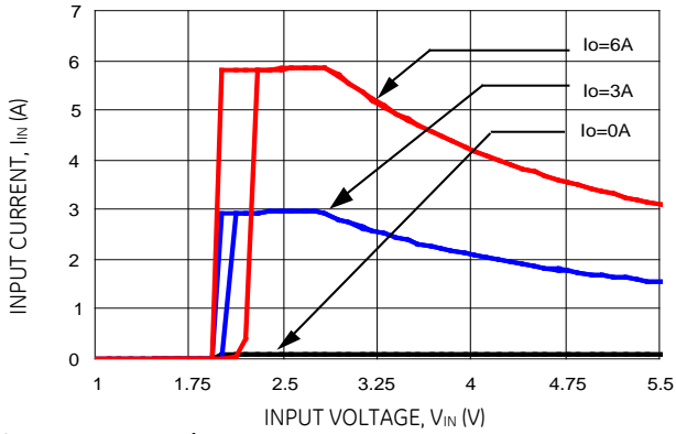
Figure 7. Input voltage vs. Input Current (V out = 2.5Vdc).
