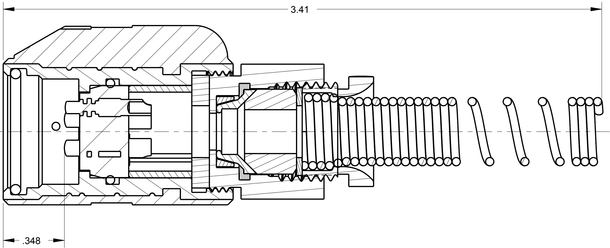
SECTION Z-Z
