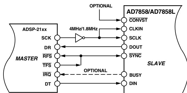
Figure 39. ADSP-21xx Interface
