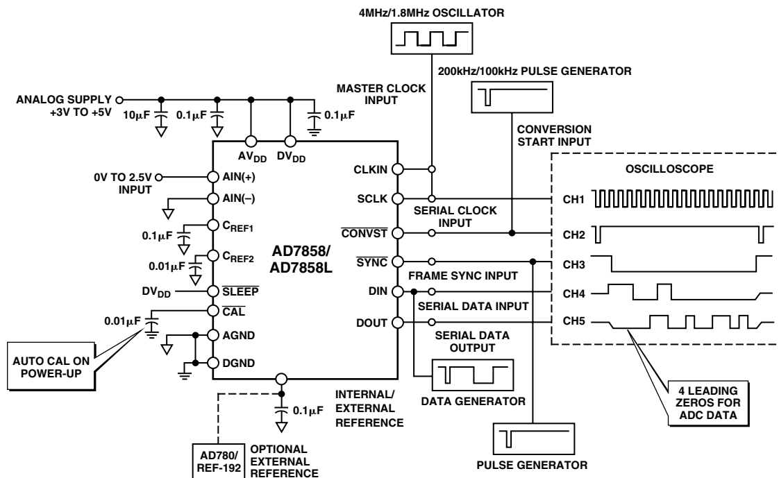
Figure 10. Typical Circuit
