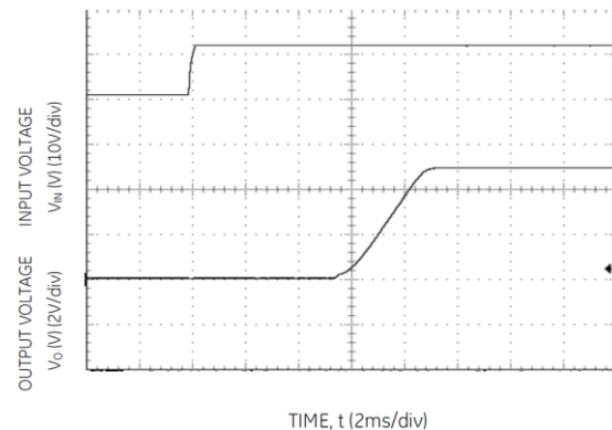
Figure 2. Typical Start-up using Input Voltage ( V_{IN} = 12\text{V} , V_{\text{out}} = V_{\text{out, max}} , I_{\text{out}} = I_{\text{out, max}} )
