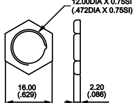
PAL NUT U42 12mm (.472") Zinc plated steel
