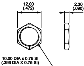
HEX CAP NUT Brass 12mm (.472") Chrome plated U35
