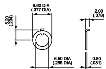
LOCKING RING 1/4 Nickel plated U78 Matte black U93
