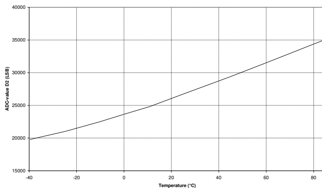
ADC-value D2 vs Temperature (typical)
