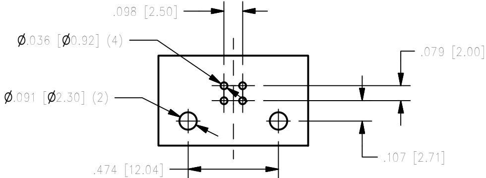
RECOMMENDED P.C.B. HOLE LAYOUT TOP VIEW (TOLERANCE ± .002 [0.05])
