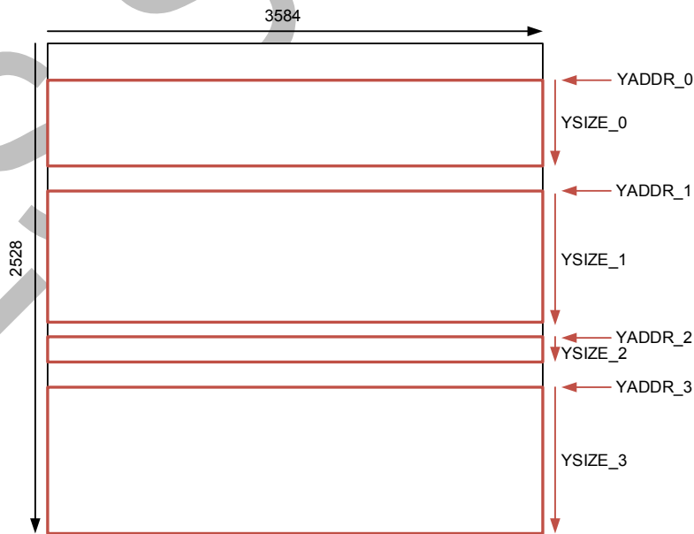
Figure 41: Example of multiple frame configuration
