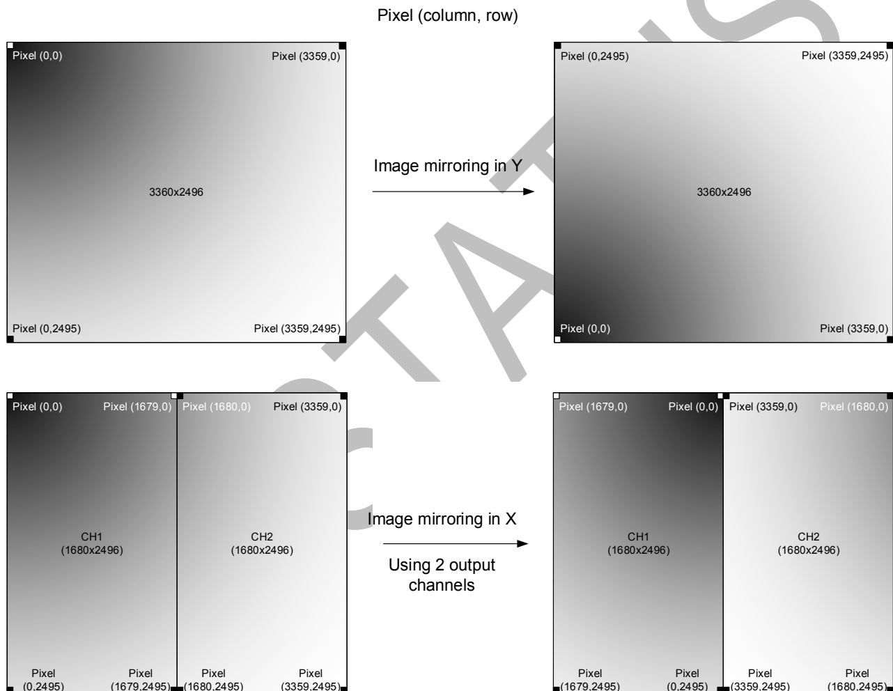
Figure 42: Image mirroring
