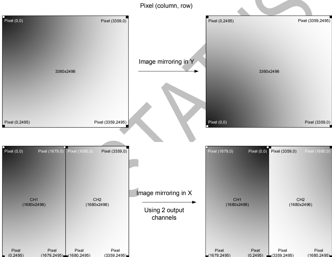
Figure 42: Image mirroring
