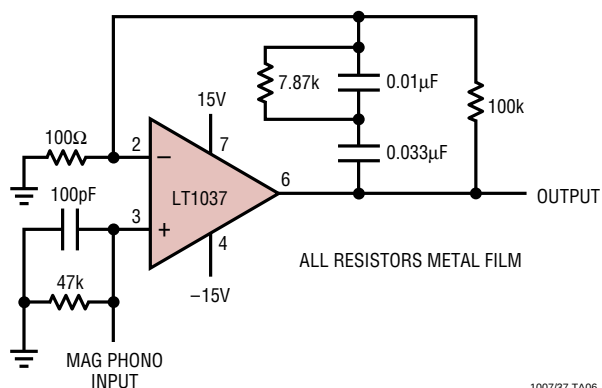
Phono Preamplifier
