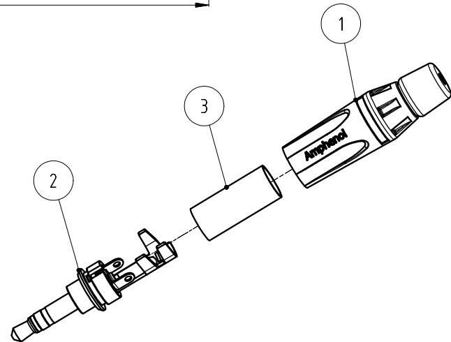
EXPLORED VIEW ( 1 : 1 )
