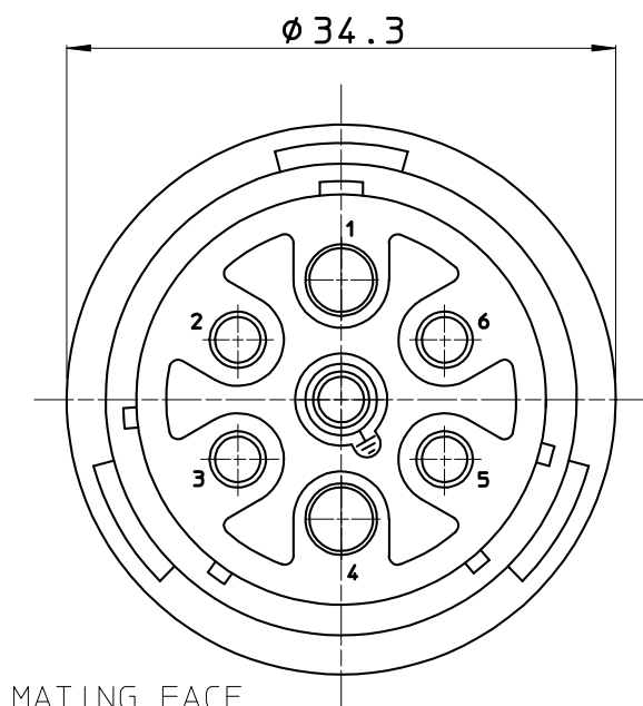
MATING FACE
