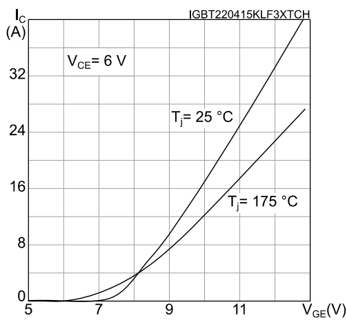
Figure 10: Transfer characteristics
